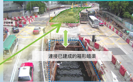
黃大仙警署附近的箱形暗渠工程 Construction of Box Culvert near Wong Tai Sin Police Station
