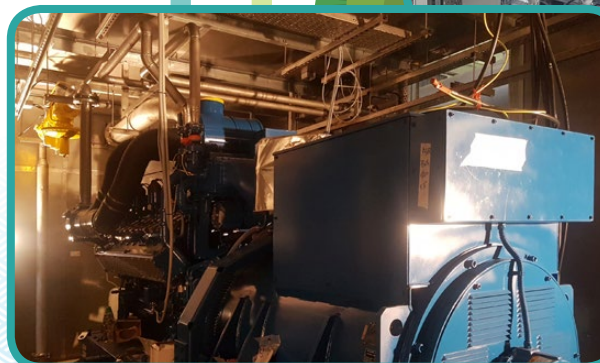
沙田污水處理廠新增的生物氣電熱聯供發電機 A new biogas-fueled combined heat and power generator at Sha Tin Sewage Treatment Works
